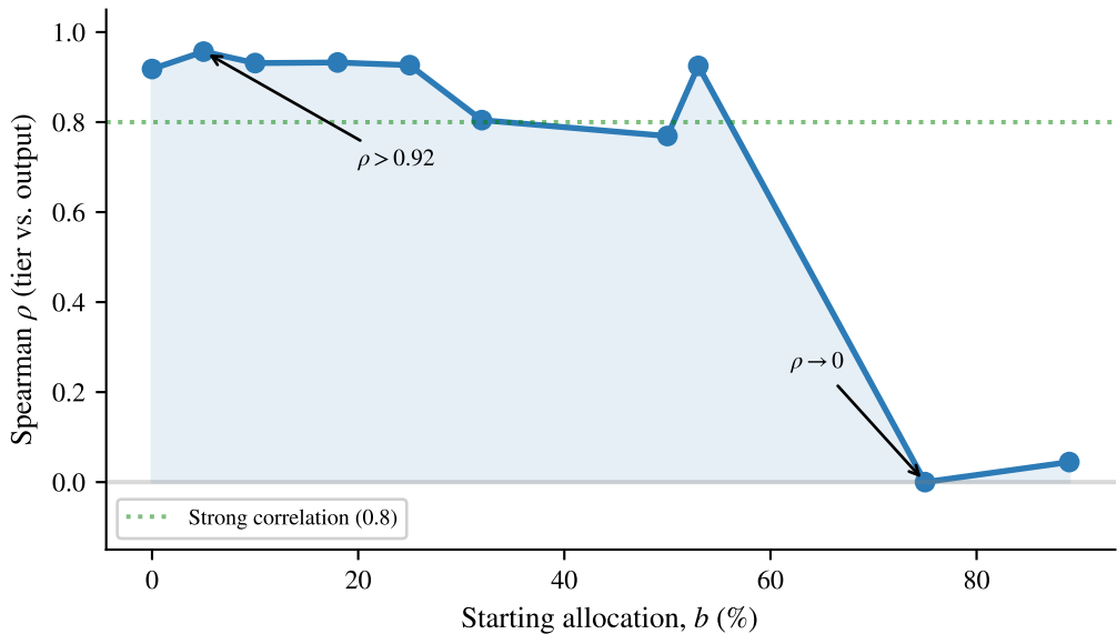
Ordinal faithfulness across baselines ( T=0.0 )
